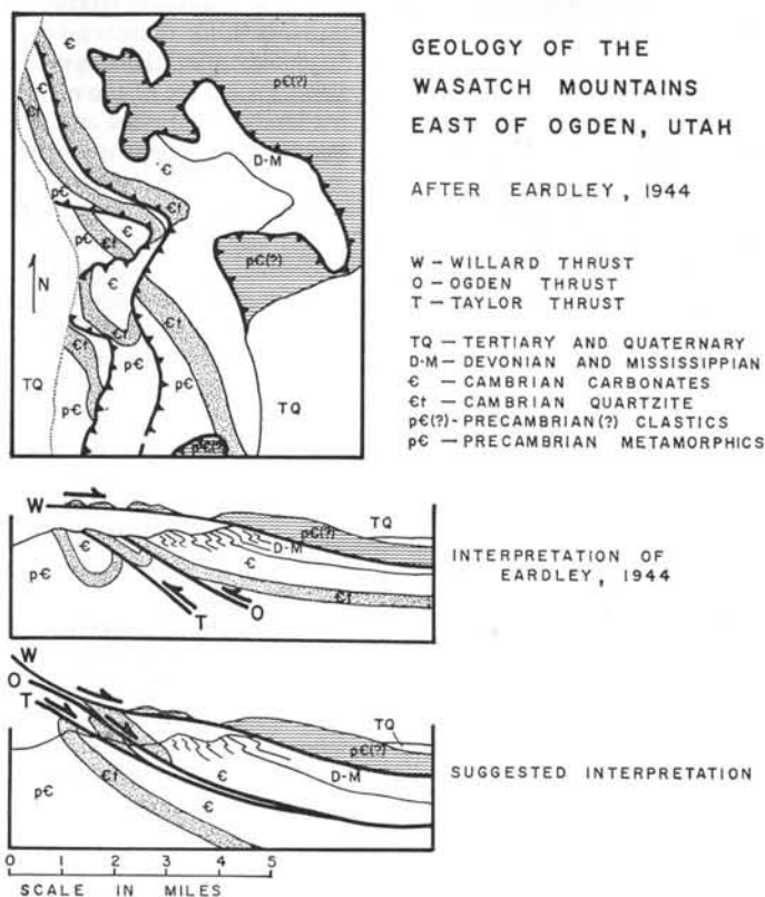
Figure 4. Reinterpretation of Taylor and Ogden thrusts.
