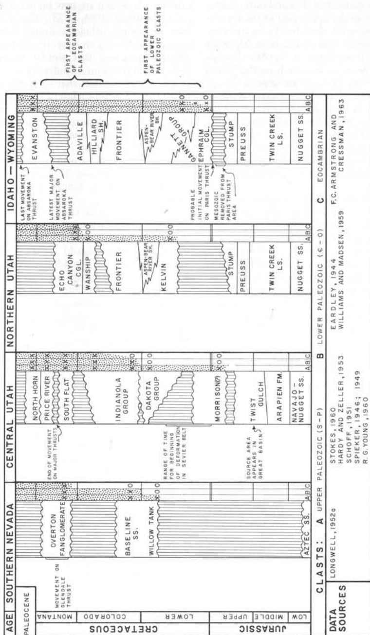
Figure 6. Jurassic to Paleocene correlation chart showing inverted stratigraphy of clasts in Rocky Mountain geosyncline.
