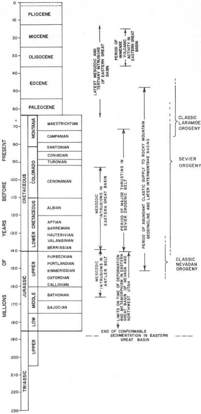
Figure 7. Geologic time scale. Tertiary time scale after Evernden and others (1964); 120 m.y. to Tertiary from work of Folinsbee and others (1960); and 230-120 m.y. modified from data given by Kulp (1961), Baadsgard and others (1961); and Armstrong (1964).
