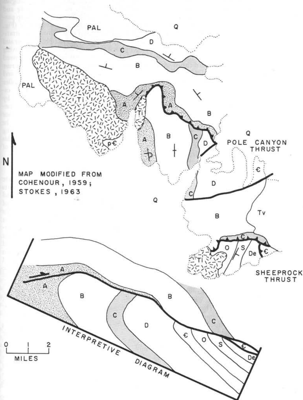
Figure 3. Relationship of Pole Canyon thrust to Sheeprock thrust, Sheeprock-West Tintic area, Utah. Pre-Lower Cambrian stratigraphic units are indicated by A , B , C , and D from bottom to top, respectively; undifferentiated Paleozoic rocks, by PAL ; Cambrian rocks, by C ; Ordovician rocks, by O ; Silurian rocks, by S ; Devonian rocks, by De ; Tertiary plutons, by Ti ; Tertiary volcanic rocks, by Tv ; and Quaternary sediments, by Q .
