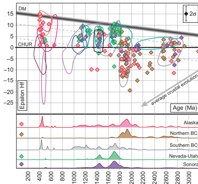
Figure 17. U-Pb and Hf isotope data from Devonian strata. Diagrams and symbols are defined in Figure 5; reference fields are defined in Figure 12. BC—British Columbia.
