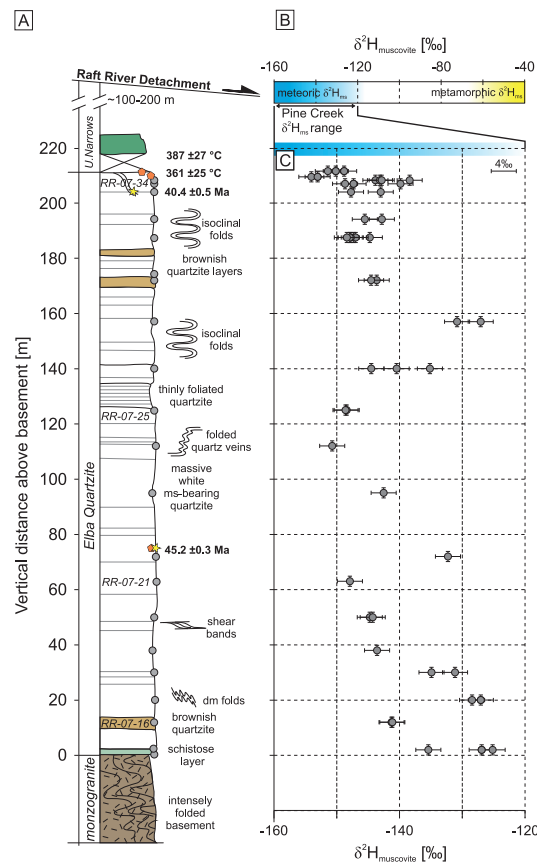
Figure 2. (a) Section of variably deformed Elba Quartzite at Pine Creek Canyon showing the location of hydrogen isotope (circles), ^{40}\text{Ar}/^{39}\text{Ar} geochronology (stars), and oxygen isotope exchange thermometry (pentagons) samples. (b) Range of typical \delta^2\text{H}_{\text{ms}} values indicative of interaction with meteoric and metamorphic fluids (notice the different scale compared to Figure 2c). (c) Muscovite hydrogen isotope values ( \delta^2\text{H}_{\text{ms}} ) of Elba Quartzite at Pine Creek Canyon. Multiple data points show replicates and different grain size fractions.
