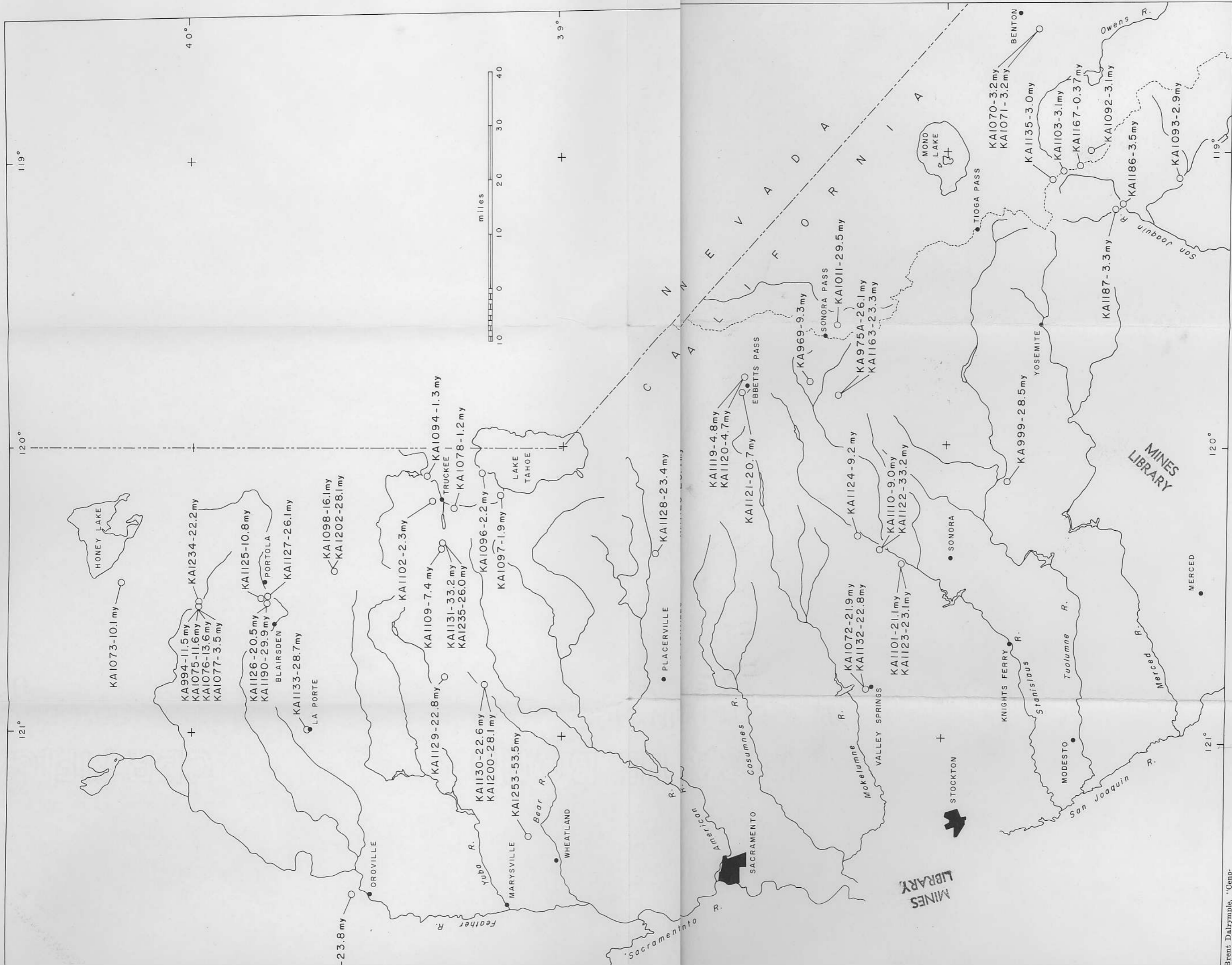
Fig. 1. Index map showing locations of dated samples.
