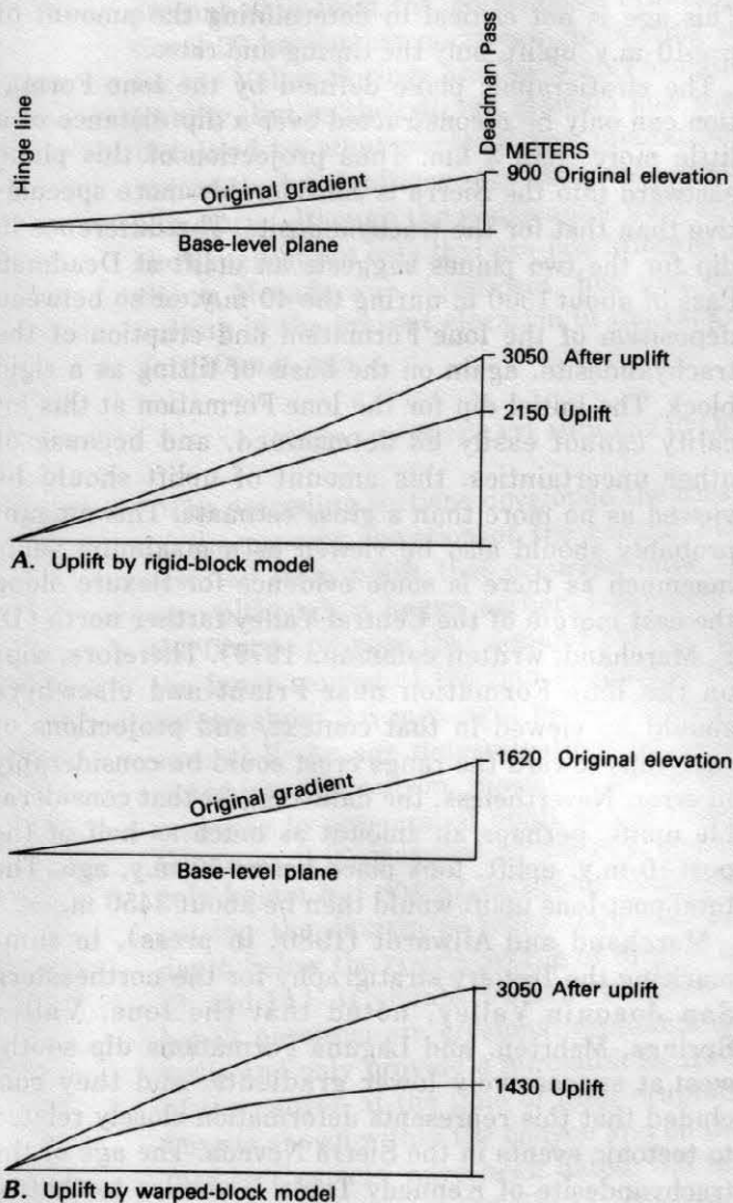
FIGURE 9.—Differences in uplift and tilt of central Sierra Nevada. Elevation of 10-m.y.-old stream profile is assumed to be 3050 m at Deadman Pass. Vertical scale and curvatures greatly exaggerated to emphasize differences. A, Rigid-block model. B, Warped-block model. Uplift for warped-block model arbitrarily reduced by one-third from that calculated for rigid-block model.
