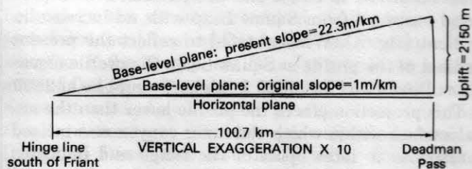
FIGURE 7.—Uplift of Sierran drainage divide at Deadman Pass calculated by rotation of late Miocene base-level plane, assuming tilting as a rigid block.
