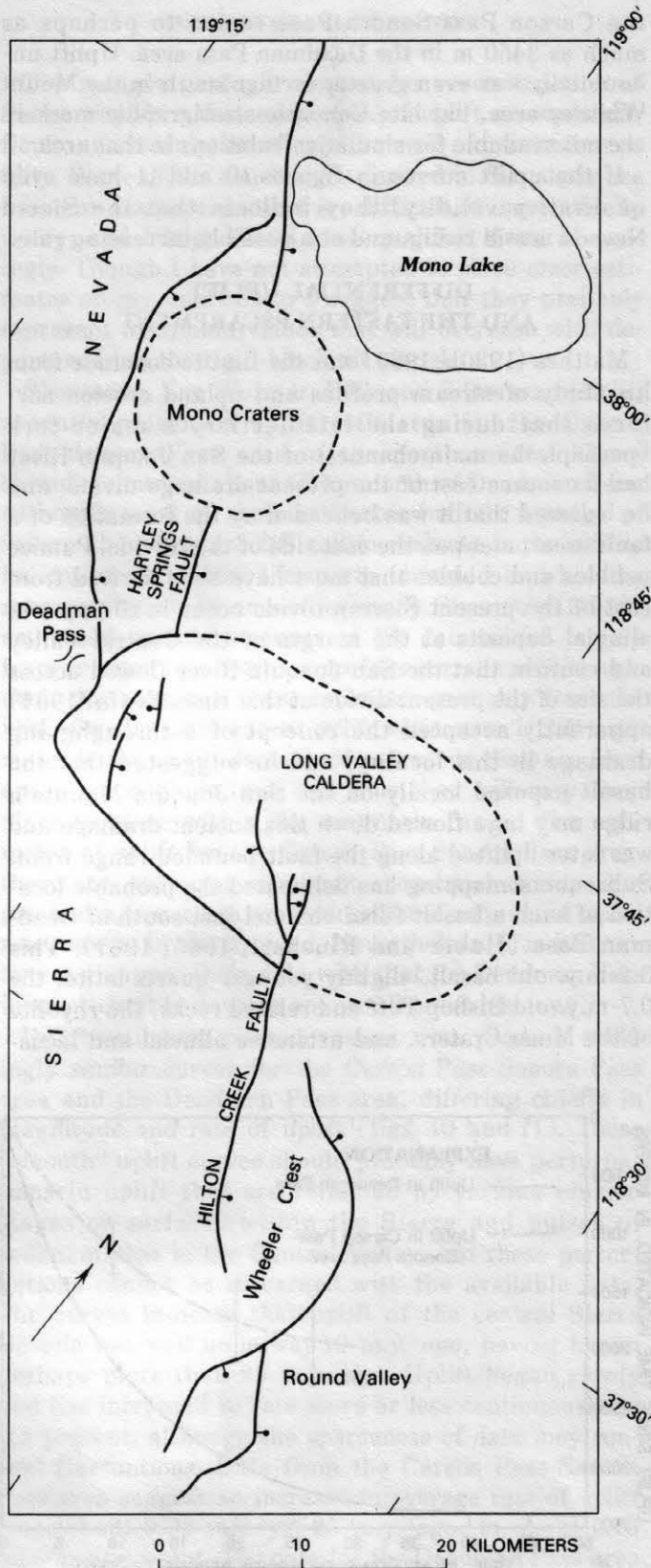
FIGURE 12.— Major faults east of Deadman Pass in Long Valley-Mono basin area. Bar and ball on downthrown side of fault. Dotted lines represent extent of Mono Craters ring structure and Long Valley caldera. After Bailey and others (1976).
