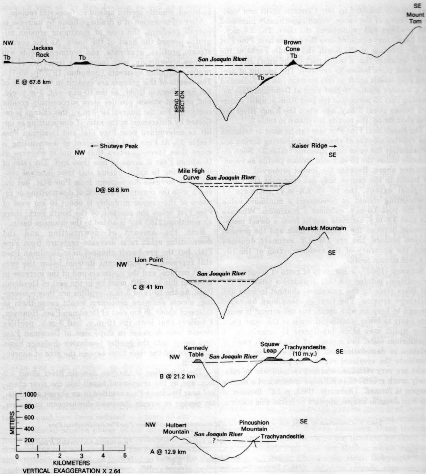
FIGURE 14.—Cross sections of San Joaquin River canyon in Sierra Nevada. Projected distances from hinge line indicated for each section (see fig. 13 for location). Section J is view of west face of Deadman Pass ridge and shows basalt-filled Pliocene channel crossing present divide south of Deadman Pass. On sections C through J, short-dash line indicates 10-m.y.-old Miocene stream profile reconstructed with no increase in gradient east of Squaw Leap; long-dash line profile with elevation of 3050 m (10,000 ft) at Deadman Pass. Actual profile assumed to lie between these lines. Section I shows fault with arrows showing direction of relative movement. Tb, Pliocene basalt.
