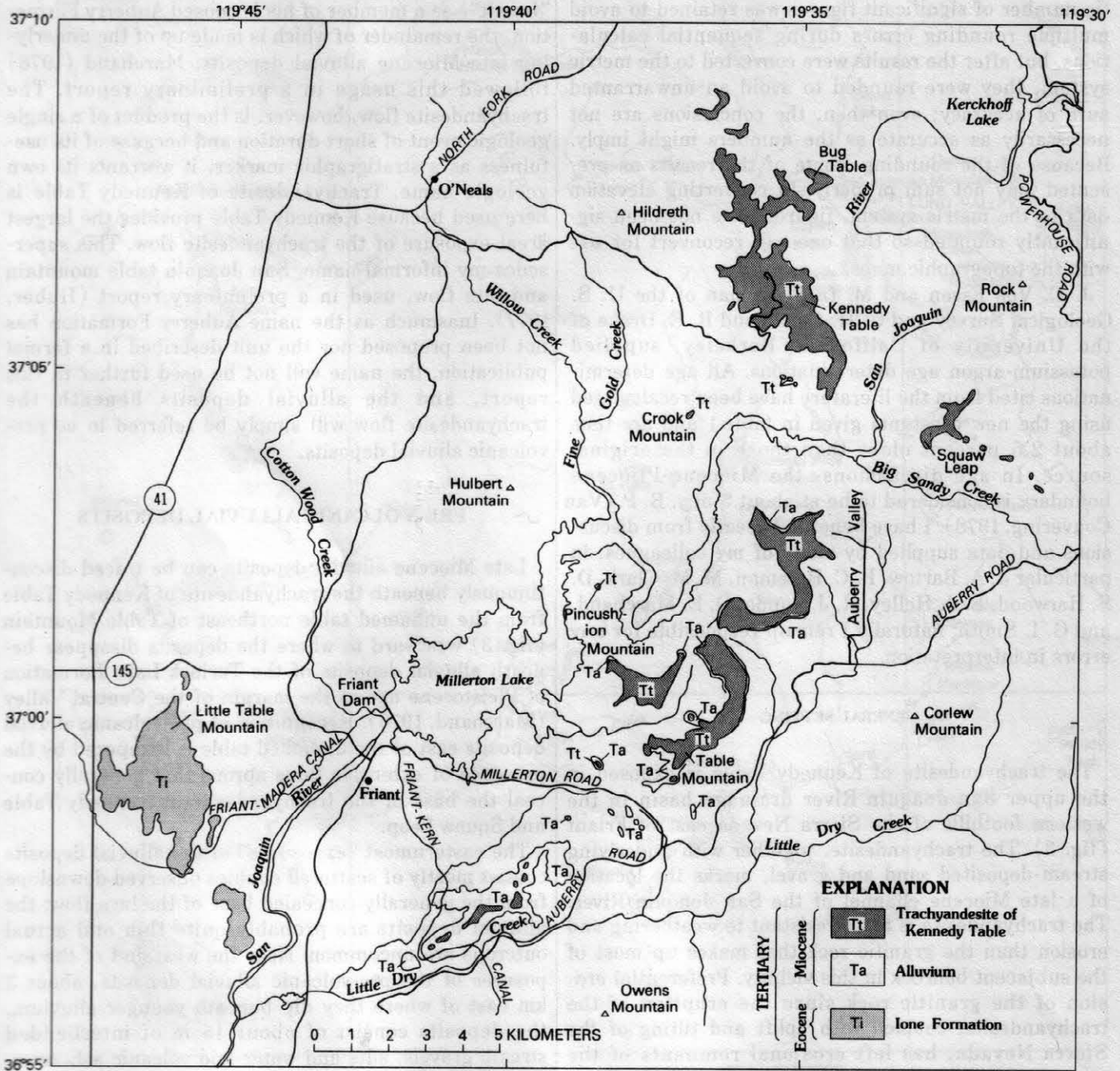
FIGURE 3.—Distribution of Tertiary units in Friant area. Modified from Macdonald (1941), Marchand (1976), and Bateman and Busacca (1980, in press).
