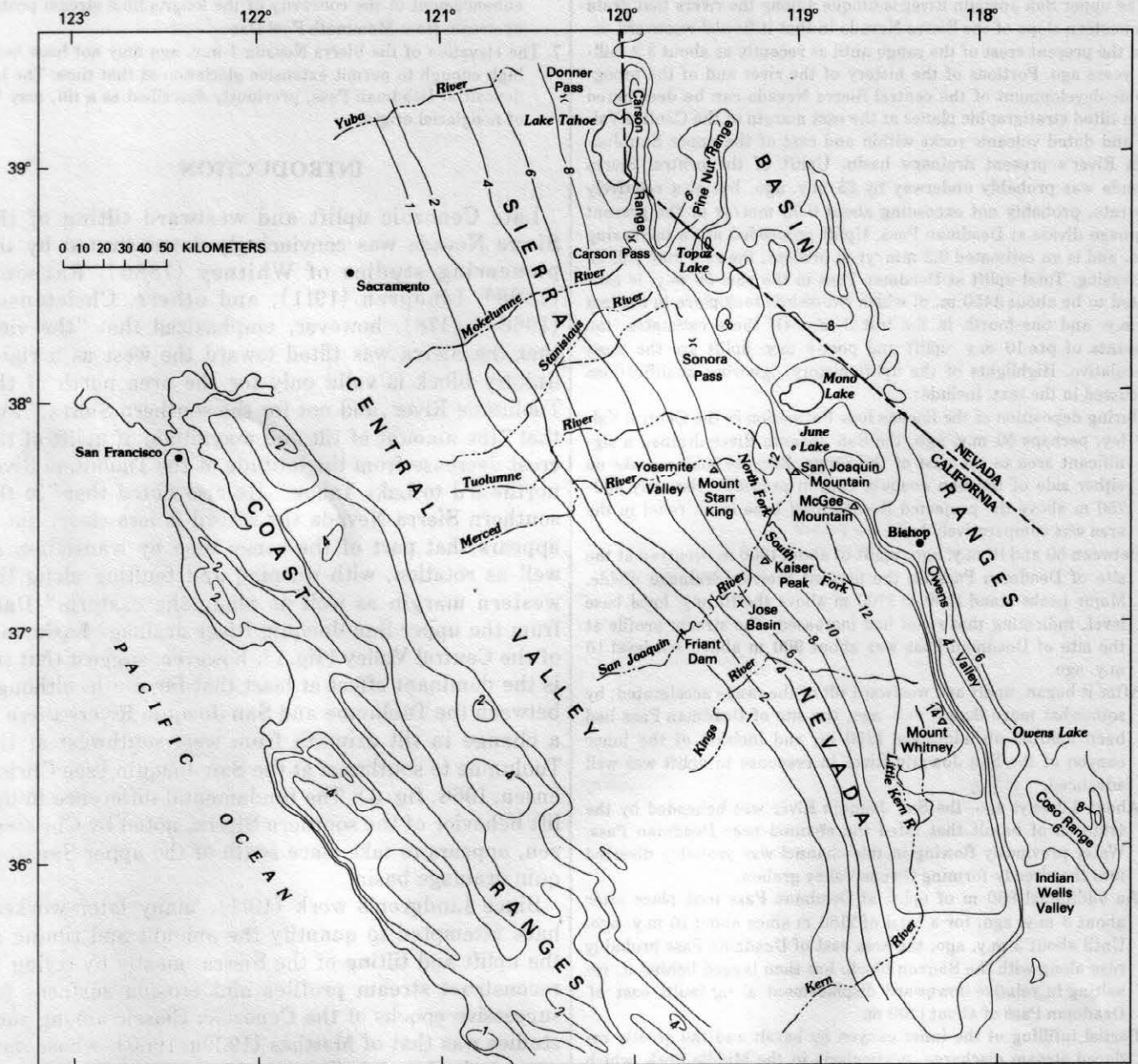
FIGURE 1.—Generalized topographic contour map of central California. Contour interval 2000 ft (610 m); 1000-ft (305 m) contour is supplementary. From Christensen (1966). "Upper" San Joaquin River is that part east of Central Valley.
