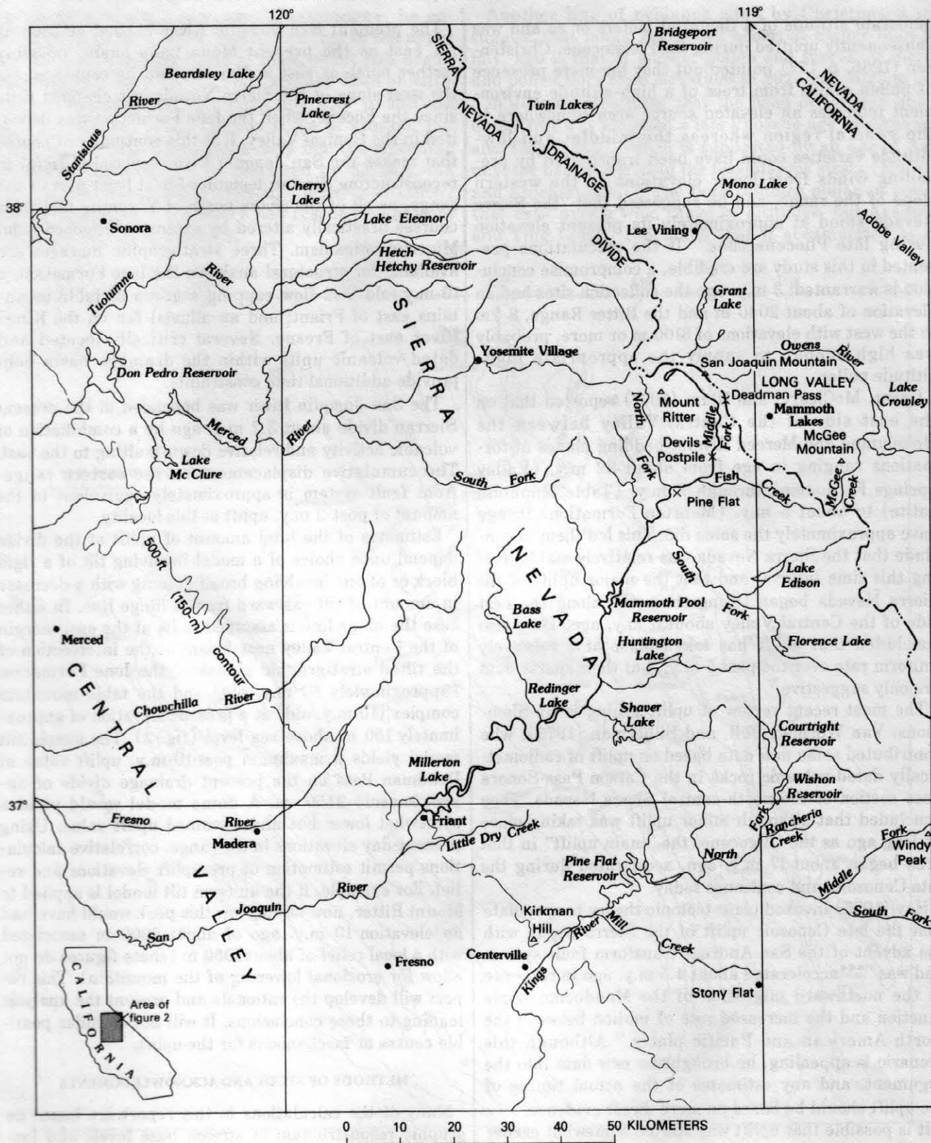
FIGURE 2.—"Upper" San Joaquin River and vicinity. The 500-ft (150-m) contour marks approximate east margin of Central Valley and assumed hinge line for Sierran tilt. Main trunk of upper San Joaquin river emphasized by heavier line weight.
