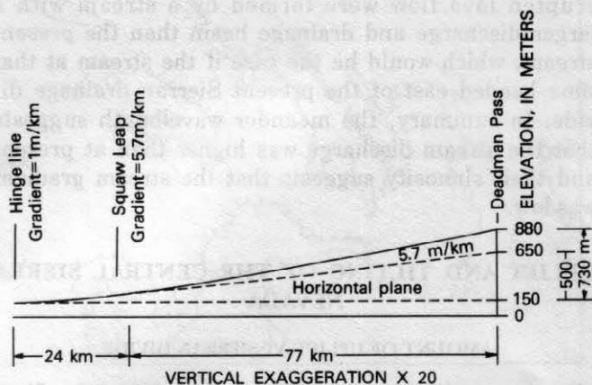
FIGURE 8.—Reconstruction of 10-m.y.-old profile of upper San Joaquin River projected to vertical plane striking N. 40° E. Elevation drop of 730 m between Deadman Pass and hinge line allows for increase in gradient east from Squaw Leap whereas 500-m drop does not.
