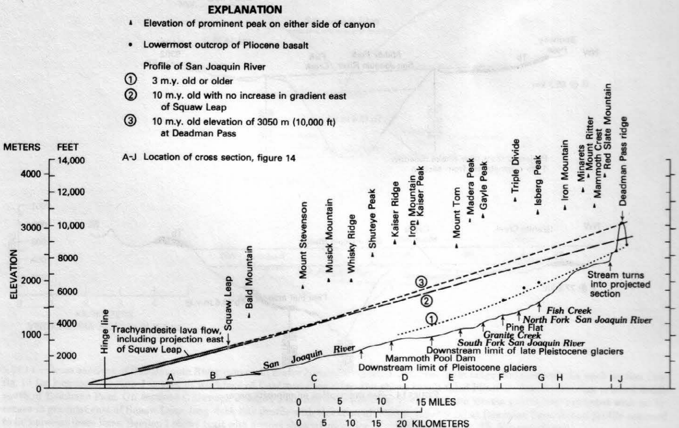
FIGURE 13.—Longitudinal profile of San Joaquin River in Sierra Nevada, projected onto vertical plane striking N. 40° E. Reconstructed profiles for late Miocene and Pliocene channels also shown.
