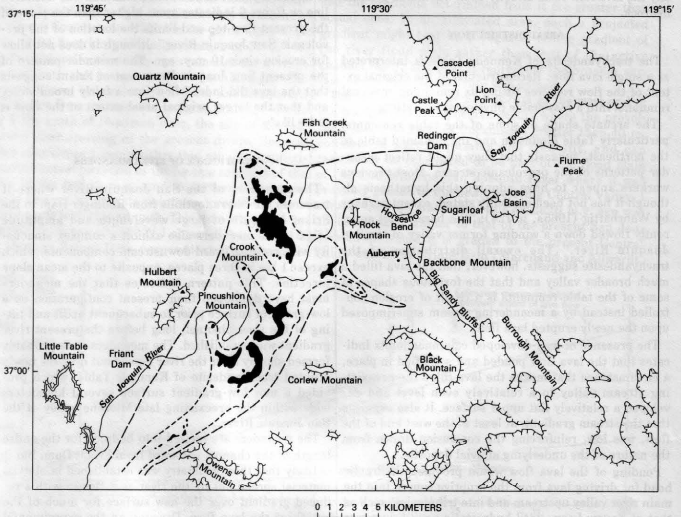
FIGURE 6.—Postulated original extent of trachyandesite of Kennedy Table. Dark areas show present outcrop; short-dash line indicates minimum extent; long-dash line probable extent. Hachured line indicates areas presently above plane defined by top of
