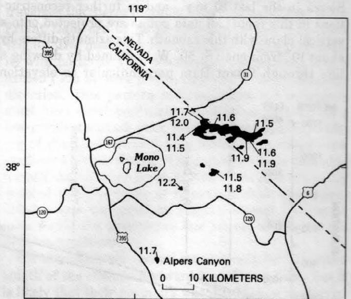
FIGURE 4.—Distribution and radiometric ages of quartz-latite welded tuff in "11-m.y." age group east of Mono Lake (Gilbert and others, 1968). Ages indicated have been recalculated using new decay constants. Alpers Canyon is location of rhyolite welded tuff (table 1).
