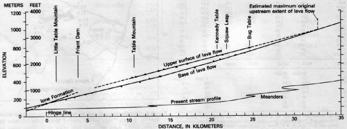
FIGURE 5.—Reconstruction of upper and lower surfaces of trachyandesite of Kennedy Table. Also shown is projection of conglomerate horizon in Ione Formation and present-day profile of San Joaquin River. All data are projected onto a vertical plane striking N. 40° E. Vertical exaggeration about 10 X.
