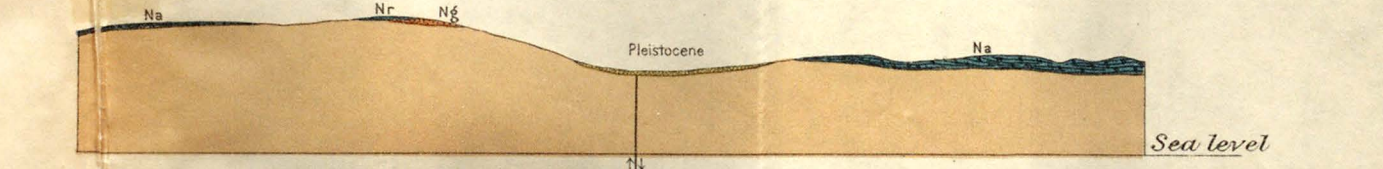
SECTION ACROSS MOHAWK VALLEY, DOWNIEVILLE QUADRANGLE Showing gravels on Haskell Peak and down-faulted eastern block
