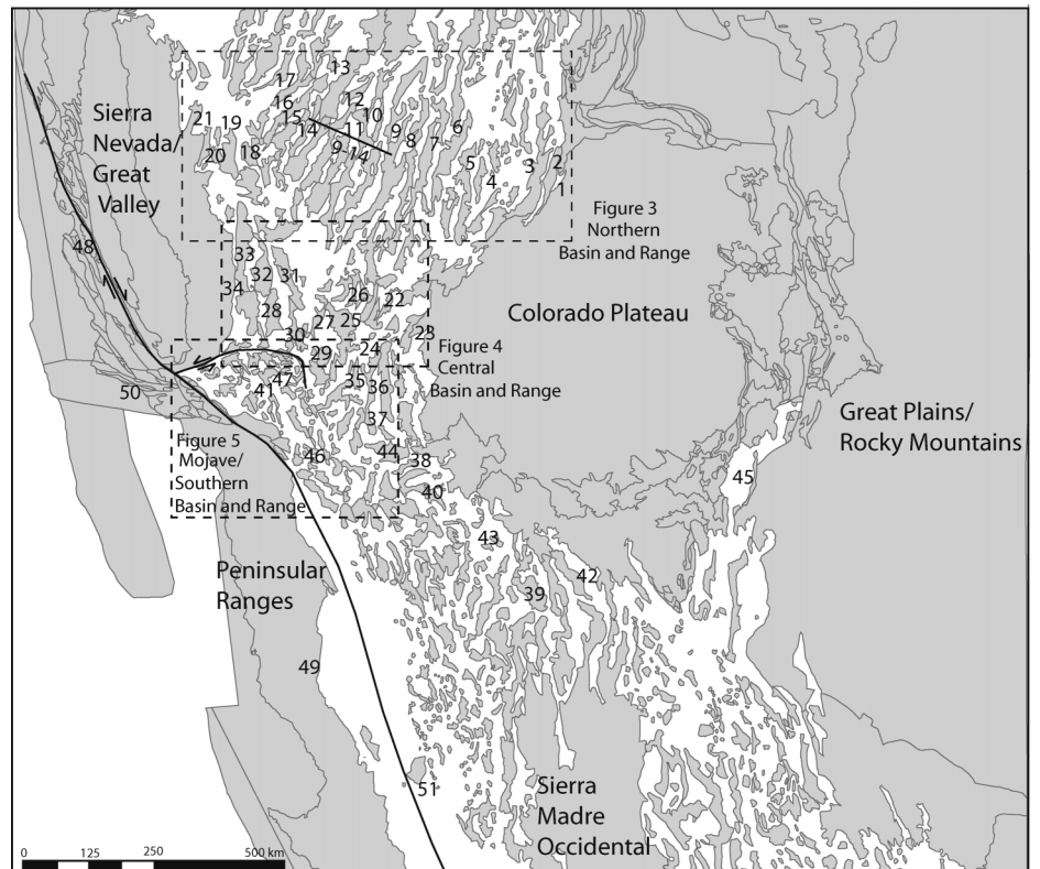
Figure 2. Map of western North America showing the primary tectonic elements in the reconstruction. The gray shaded polygons represent the physiographic or geologic expression of mountain ranges, which in the Basin and Range are fault bounded and separated by alluvial valleys. Dashed boxes are the locations of Figures 3–5. The numbers refer to specific mountain ranges identified in Tables 1–6.
