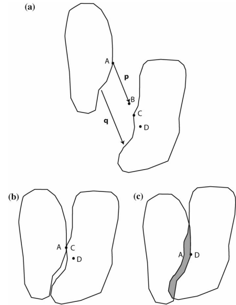
Figure 1. Schematic diagram illustrating the method of using regional structural constraints to limit possible displacement paths in tectonic reconstructions. See text for discussion and explanation of letters.
