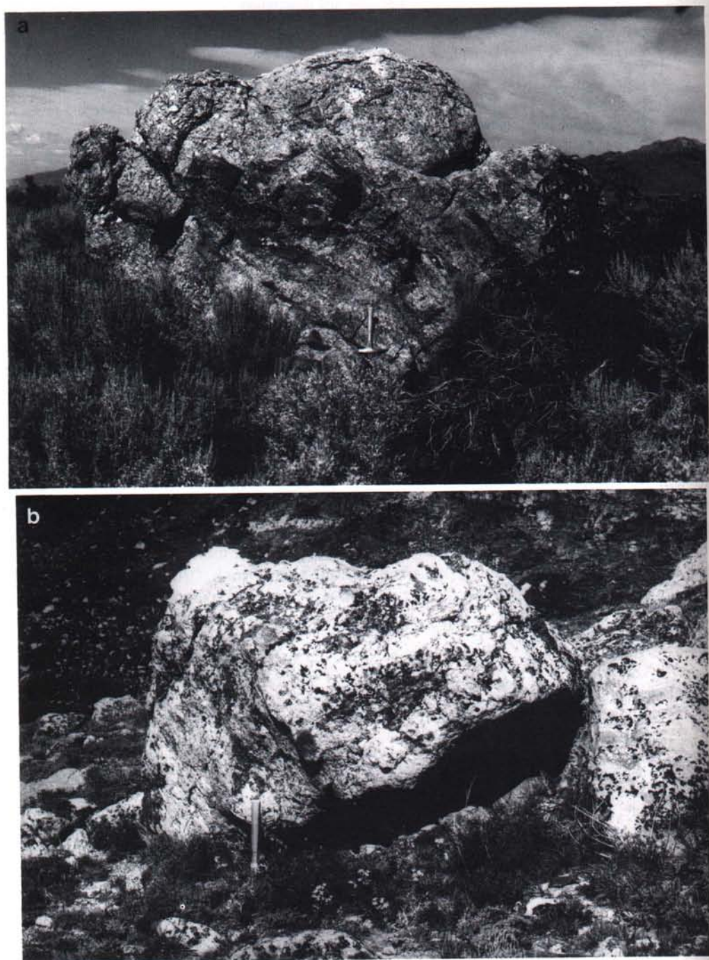
FIG. 6. Granitic-boulder weathering. (a) Boulder on crest of Lamoille Stage moraine below mouth of Lamoille Canyon. (b) Boulder on crest of outermost Angel Lake moraine at mouth of first valley south of Angel Lake.
