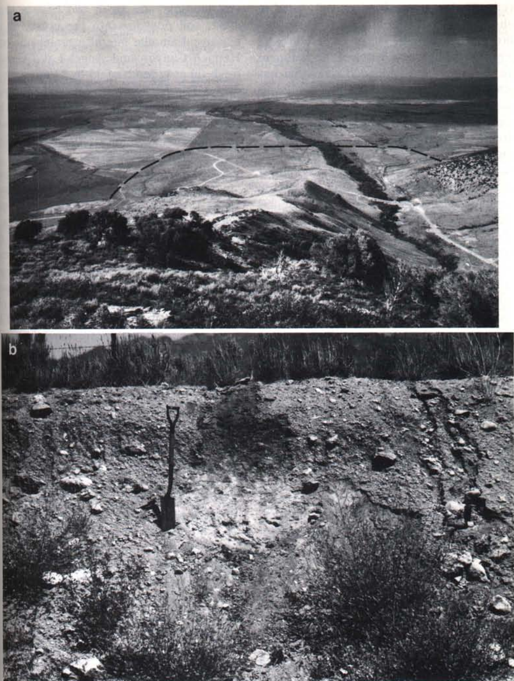
FIG. 4. Lamoille end moraine and outwash pattern, and soil profile on Lamoille till. (a) Drainage pattern on Lamoille outwash beyond end moraines at Lamoille canyon; dashed line marks boundary between till and outwash. Angel Lake outwash is confined to tree-covered strip along Lamoille Creek. (b) Soil profile on Lamoille Stage till in road cut through outermost end moraine.
