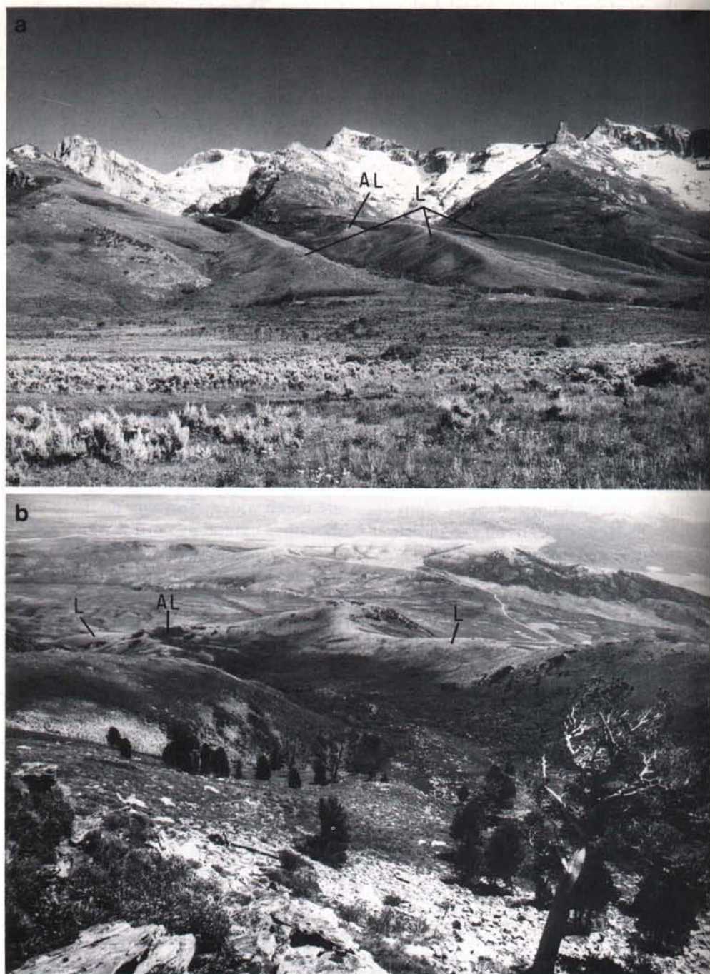
FIG. 3. Lamoille (L) and Angel Lake (AL) morainal topography. (a) Hennen Canyon. Fault scarp base marked by line of trees; top of fan below scarp is Lamoille end moraines nearly obscured by Angel Lake outwash. (b) Valley north of Angel Lake. Only a few small moraines are found in most valleys above the well-developed end moraines of the Angel Lake glaciation.
