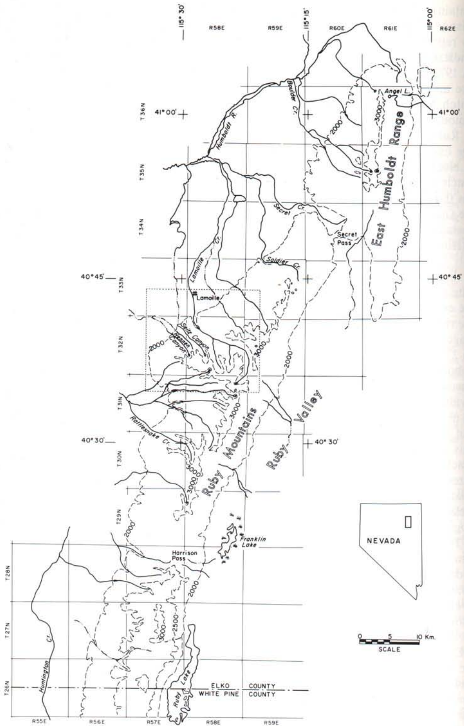
FIG. 1. Index map of East Humboldt Range and north part of the Ruby Mountains showing 1000-m contours and major drainage lines. Outline shows area of Figure 2. From U.S. Geological Survey Elko and Wells quadrangles, scale 1:250,000.
