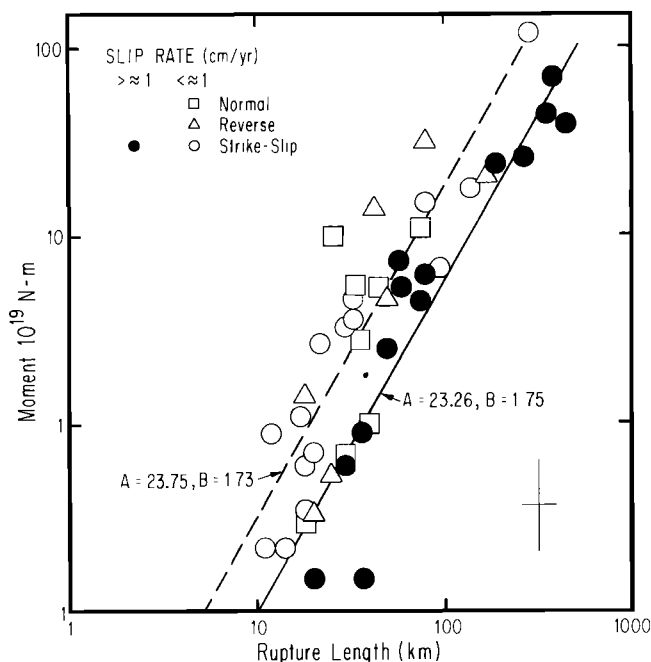
Fig. 2. Seismic moment M_0 versus rupture length l for earthquakes listed in Table 2. Solid symbols indicate earthquakes on major plate boundary faults generally characterized to have slip rates of 1 cm/yr or greater. Earthquakes on faults with lesser slip rates are shown by open symbols. Lines of form \log M_0 = A + B \times \log l are fit through the solid and open symbols, respectively. Squares, triangles, and circles correspond to normal, reverse, and strike-slip type earthquakes, respectively. The vertical and horizontal bars of the cross in lower right corner of plot correspond to a factor of 3 in M_0 and 50% in l , respectively.
