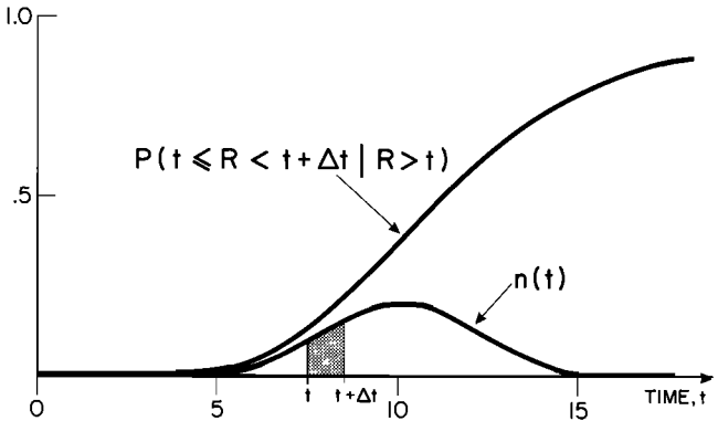
Fig. 5. The conditional probability that a fault will rupture at time R during the period t_1 to t_2 years conditional that t_1 years are past since the time of last rupture ( R_l=0 ), for the specific case where R_p , \sigma , and t_2 - t_1 are arbitrarily taken to equal 10, 2, and 1, respectively. The standard normal probability density function n(t) for the same set of parameters is also shown.
