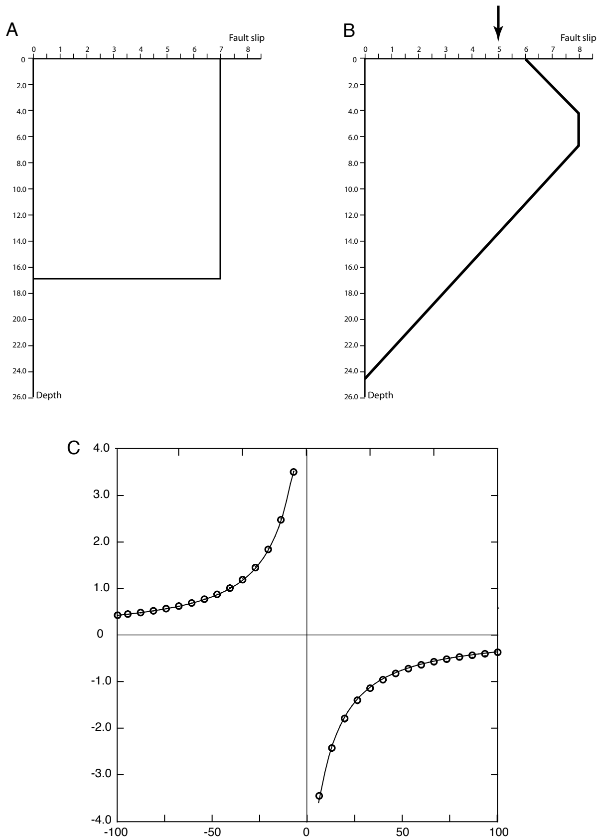
Figure 5. The (A) box and (B) tapered displacement functions produce (C) the same deformation field (circles and lines) at the earth's surface. Vertical axis is meters of surface displacement and horizontal is distance in kilometers from fault.
