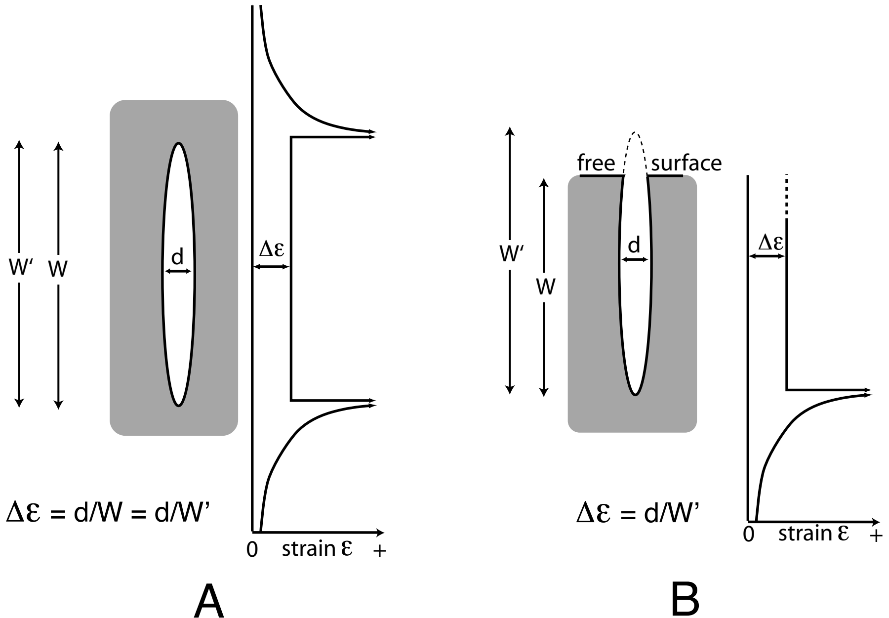
Figure 1. Strain profiles for dislocation surfaces (A) entirely and (B) partially in an elastic medium (shaded) on which an elliptical slip distribution has been imposed for each. Surfaces are of infinite length into page. Strain drop \Delta\varepsilon for each is almost identical and equal to d/W' where d is maximum displacement and W' is width (shortest dimension) of the surface. Small differences in constant strain drop (dashed line) will occur near the surface for case (B). For case (B) where the crack intersects the free surface W' is greater than the portion W of crack embedded in the medium. By analogy W is the depth to which a fault extends into the earth's crust and the endmember cases W=W' and W'=2W correspond to the definition of small and large earthquakes by Scholz (1982).
