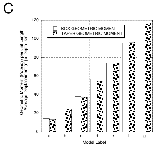
Figure 7. Comparison of (A) depth extent, (B) average displacement, and (C) the geometric moment for the paired box and tapered displacement-depth profiles shown in Figure 6.
