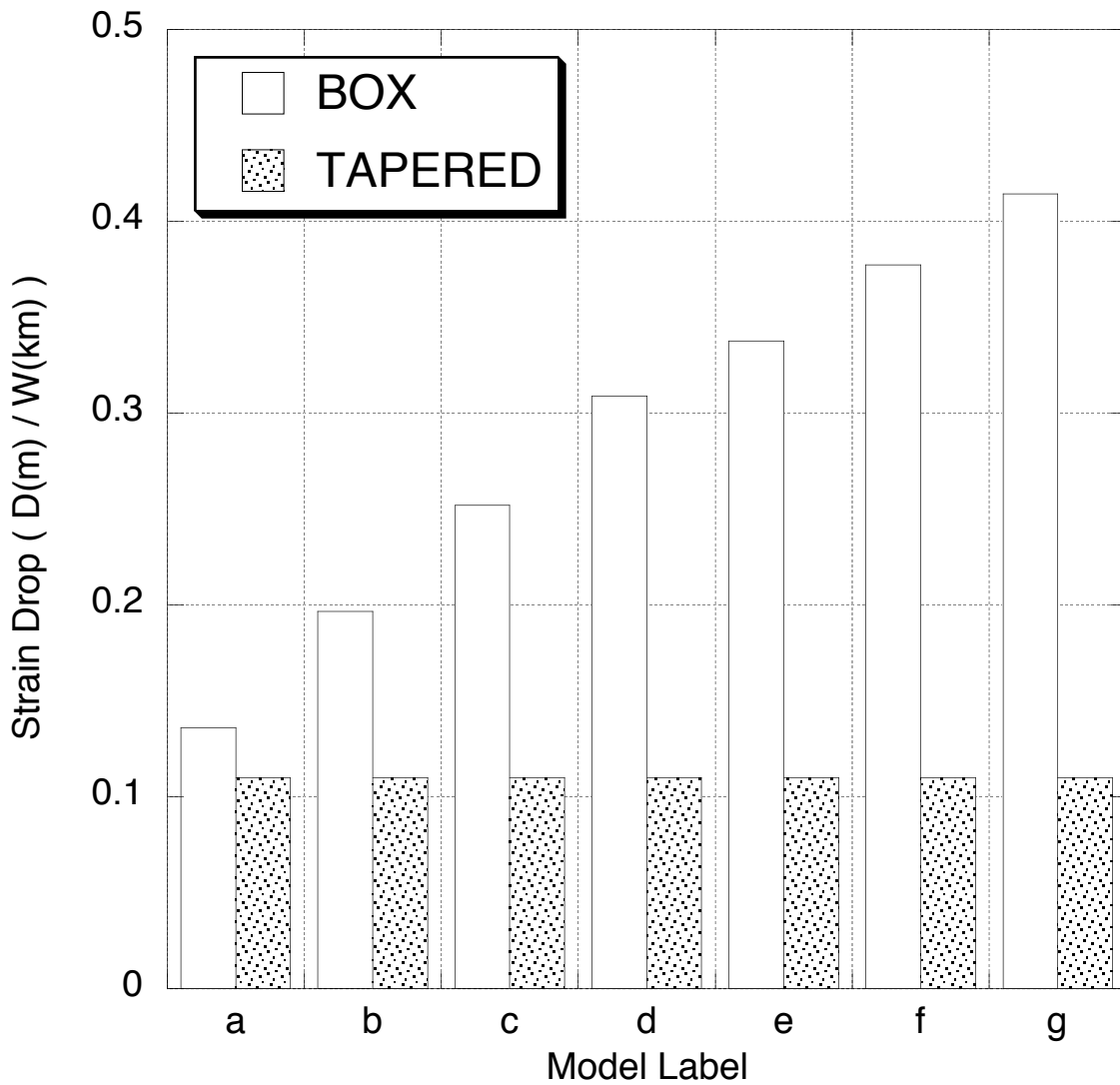
Figure 8. Comparison of values of strain drop for the paired box and tapered displacement-depth profile models in Figure 6. Strain drop increases with earthquake size for the box function but remains constant for tapered function. See text for further discussion.
