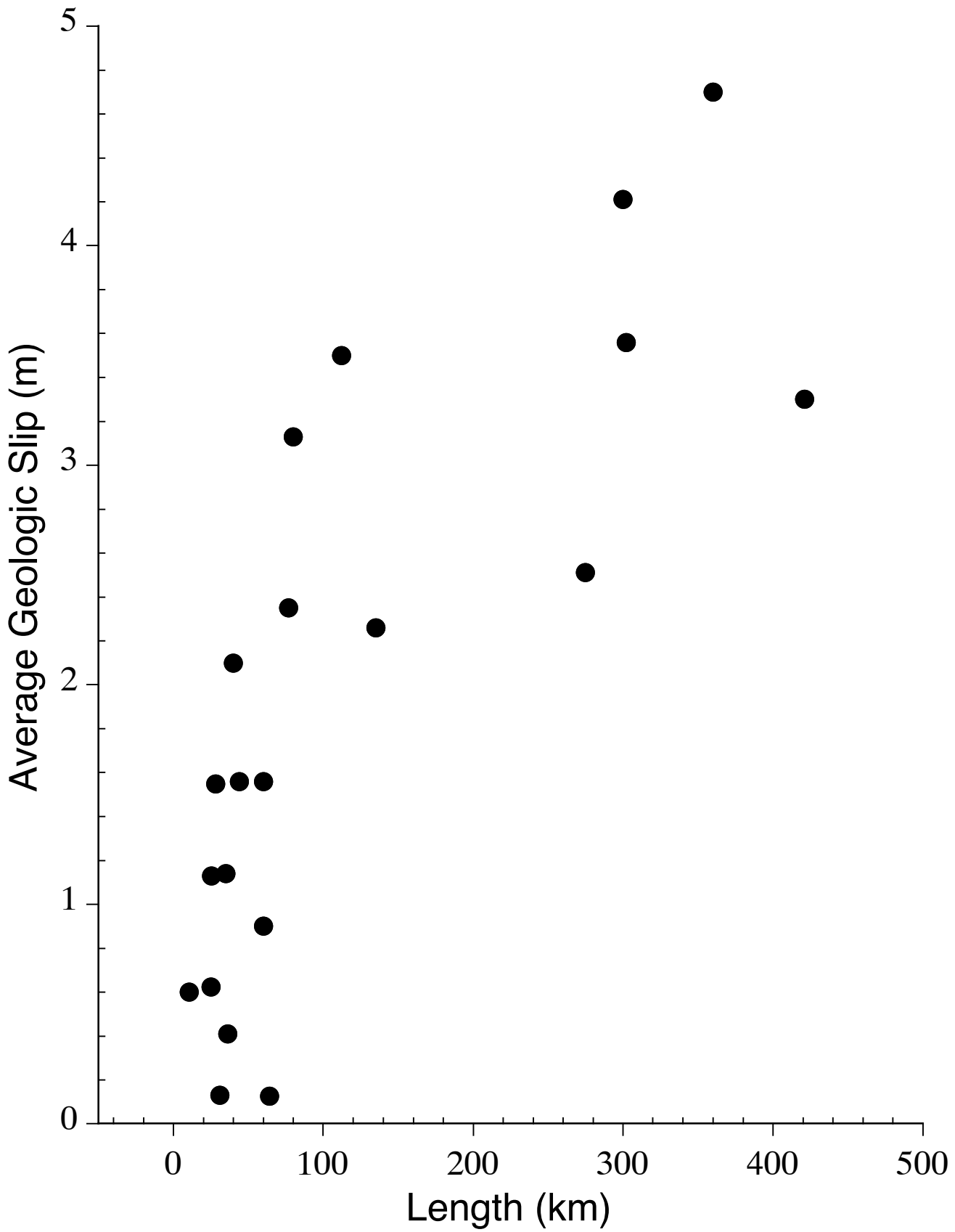
Figure 2. Average surface displacement is an increasing function of rupture length for continental strike-slip earthquakes. Adapted from Wesnousky (2007).
