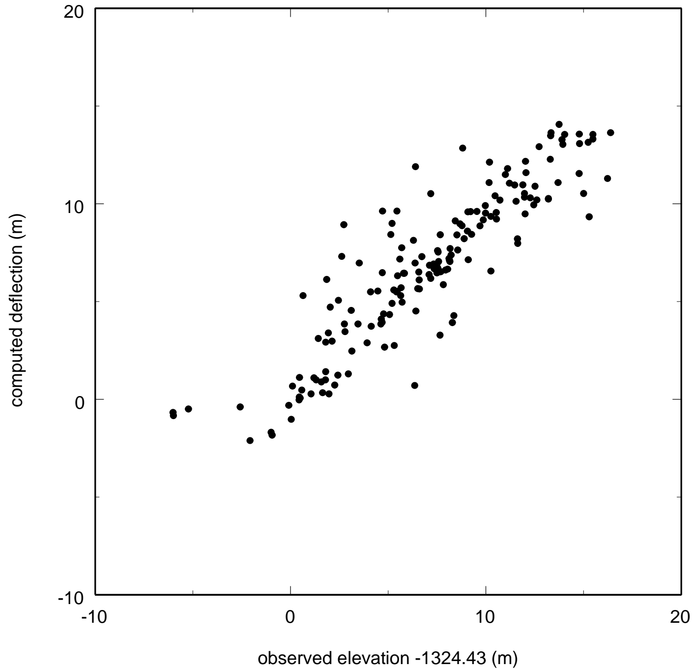
observed versus computed elevations
