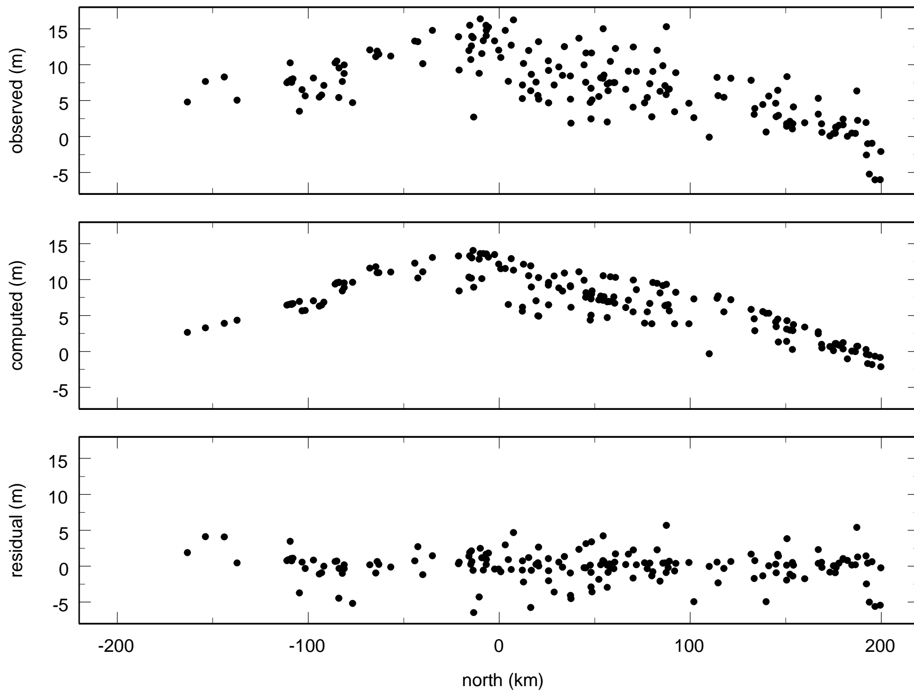
shoreline elevation pattern projected onto north-south line
