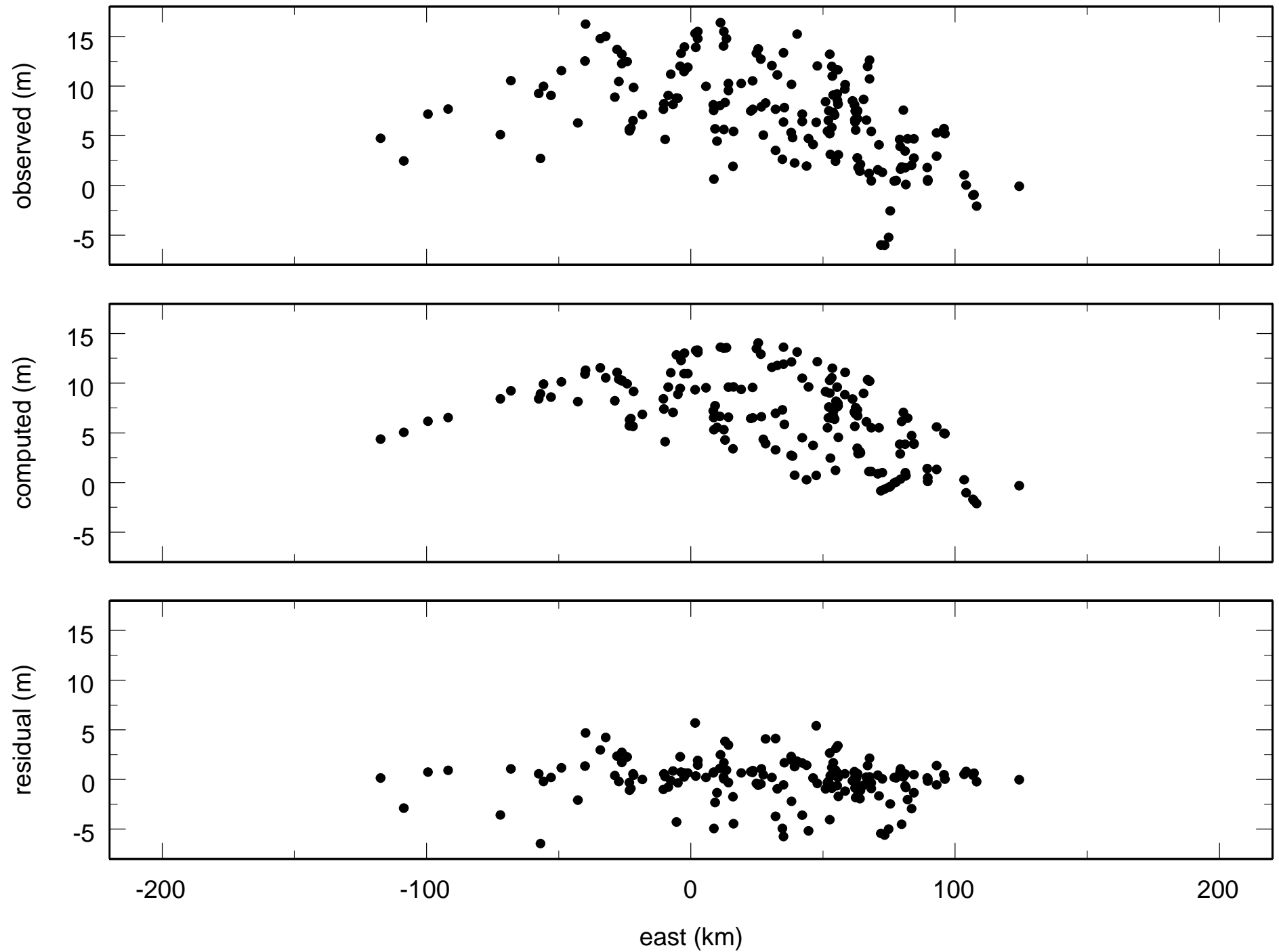
shoreline elevation pattern projected onto east-west line
